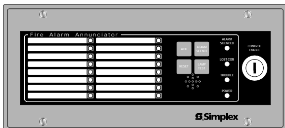
4610-9111 LED/Switch Annunciator
