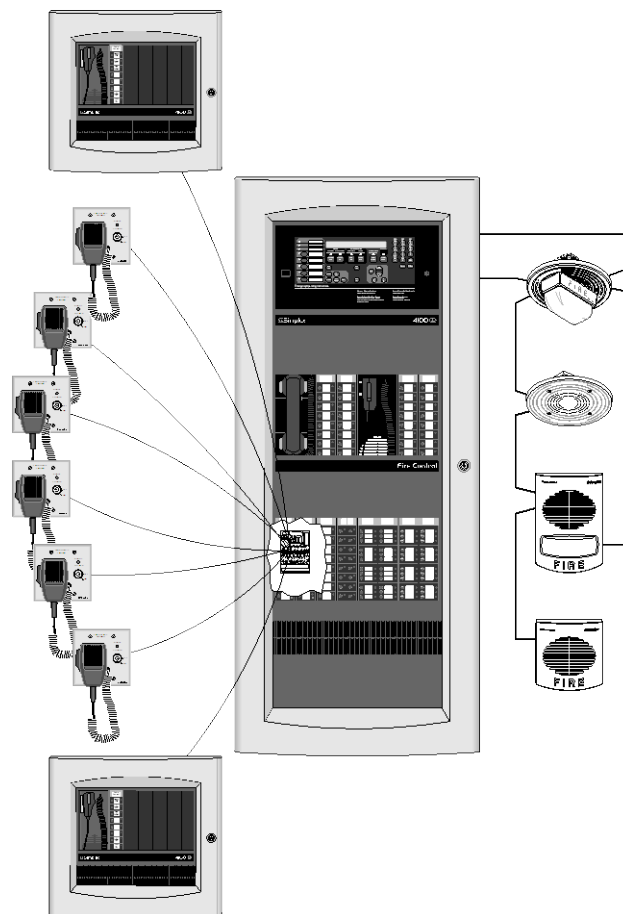
4100ES Audio System with 4100-1274 Microphone Multiplex Module and 8 Remote Microphones; 6, Model 4003-9803 Remote Microphones and 2 (single bay) Remote Annunciators with Remote Microphone
