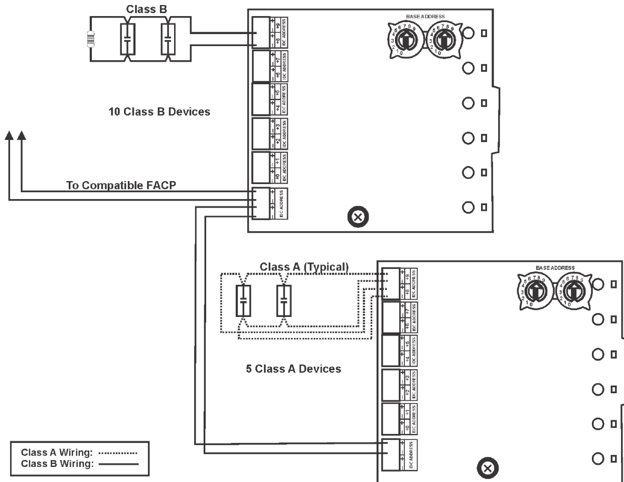
Wiring IDP-Monitor-10 Monitoring Modules
