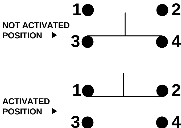
Figure 3 Contact Arrangements
