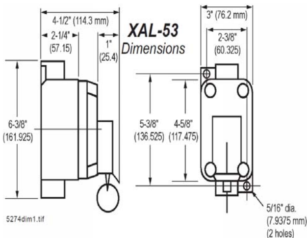
Figure 2 XAL-53 Dimensions
